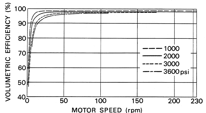
Fig.3 Volumetric Efficiency
