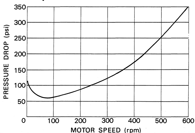
Fig.7 Pressure Drop
