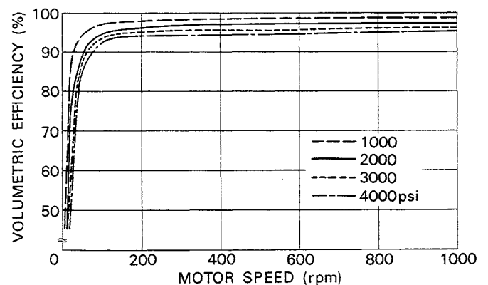
Fig.3 Volumetric Efficiency
