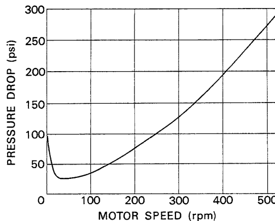
Fig.7 Pressure Drop
