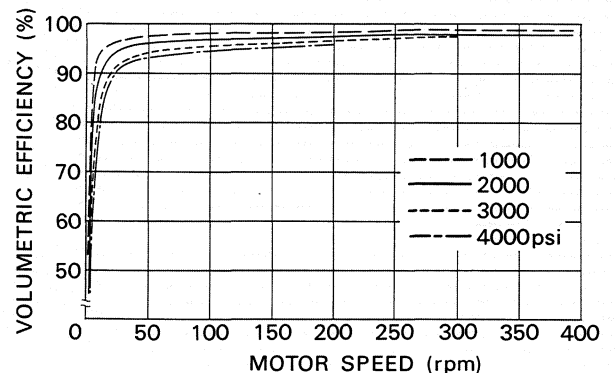
Fig.3 Volumetric Efficiency
