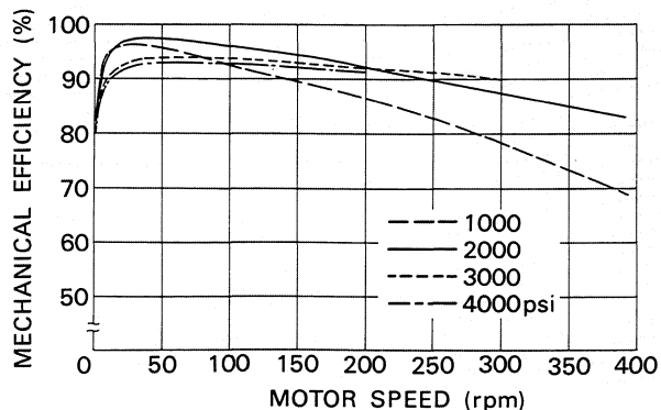
Fig.2 Mechanical Efficiency
