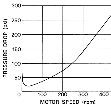
Fig. 7 Pressure Drop
