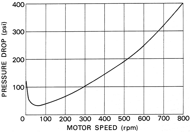
Fig.7 Pressure Drop
